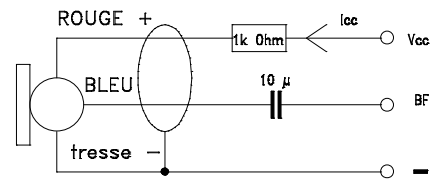
Schema de mesure Measuring diagram
